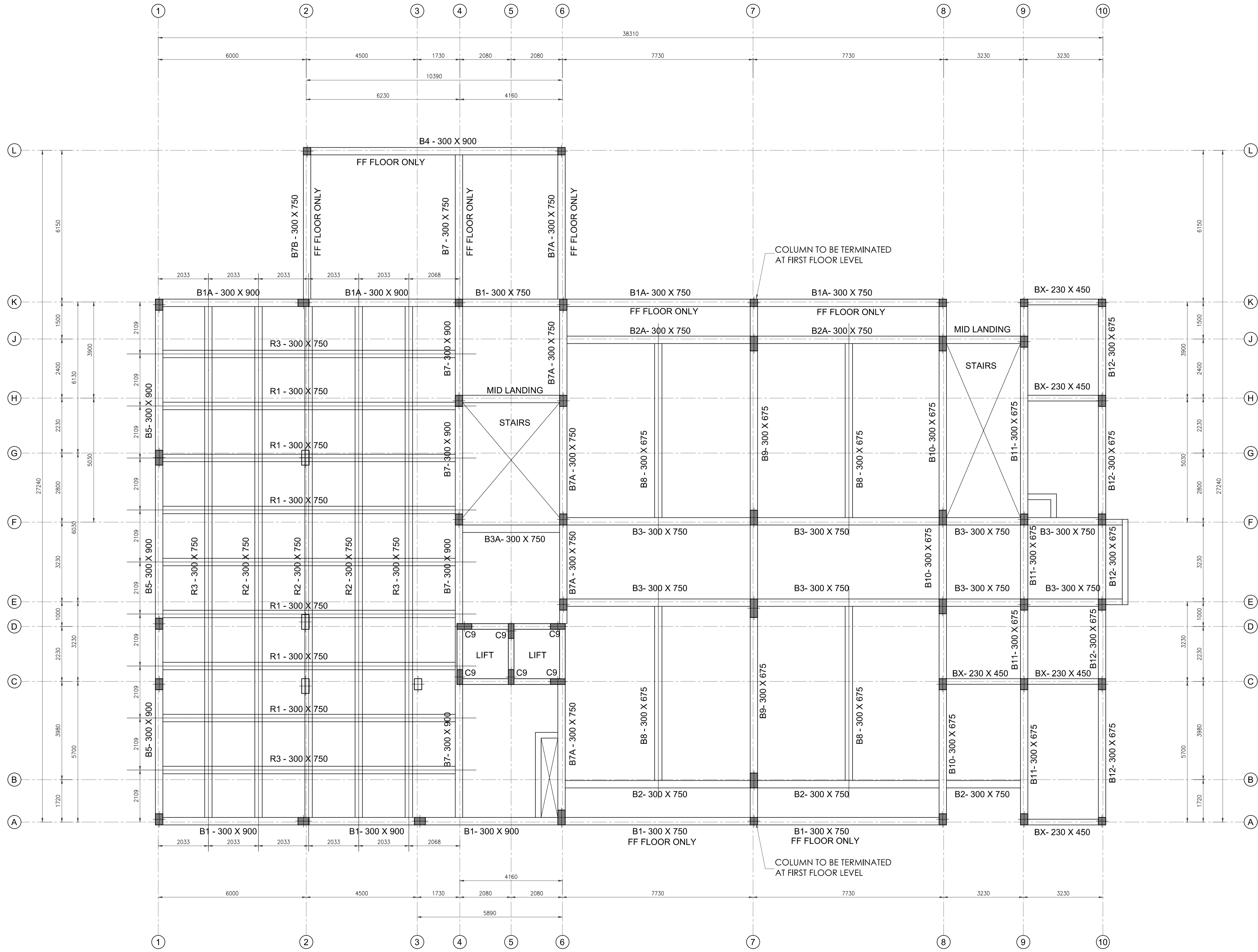
FIRST FLOOR LVL BEAM LAYOUT ALL SLABS ARE 140 THK
